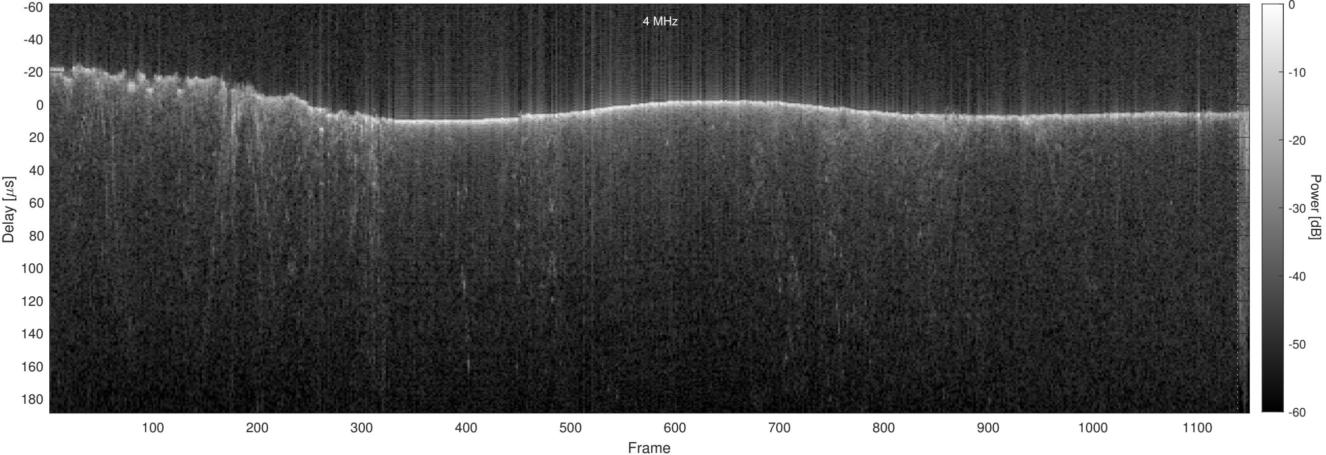
Orbit 3971, Optimized, No Window, Channel 2
