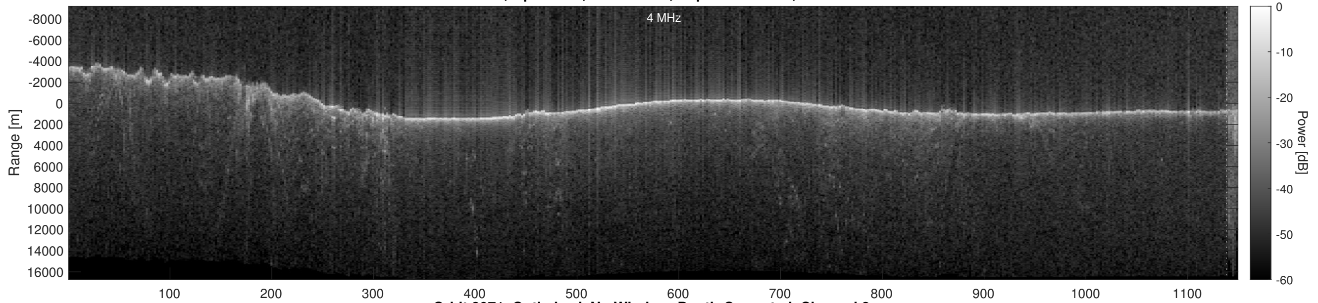
Orbit 3971, Optimized, No Window, Depth-Corrected, Channel 2
