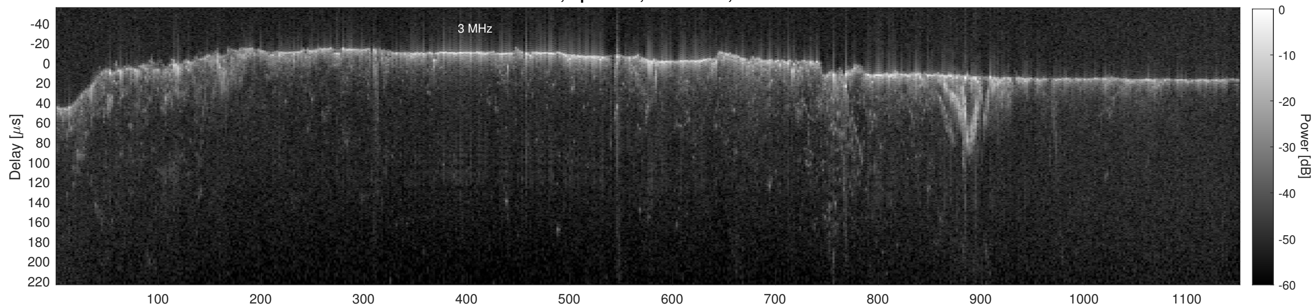
Orbit 3972, Cluttergram
