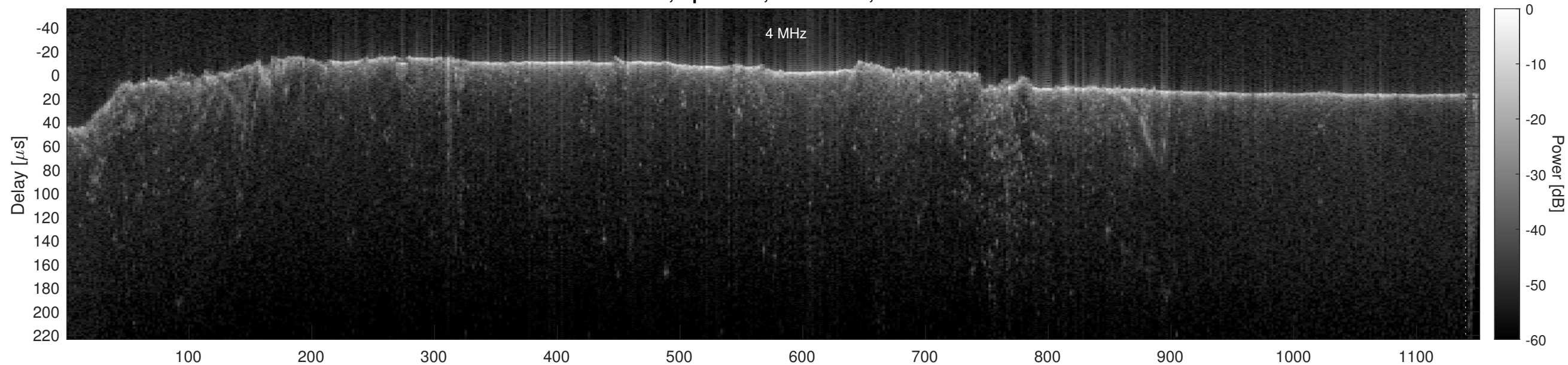
Orbit 3972, Optimized, No Window, Channel 2
