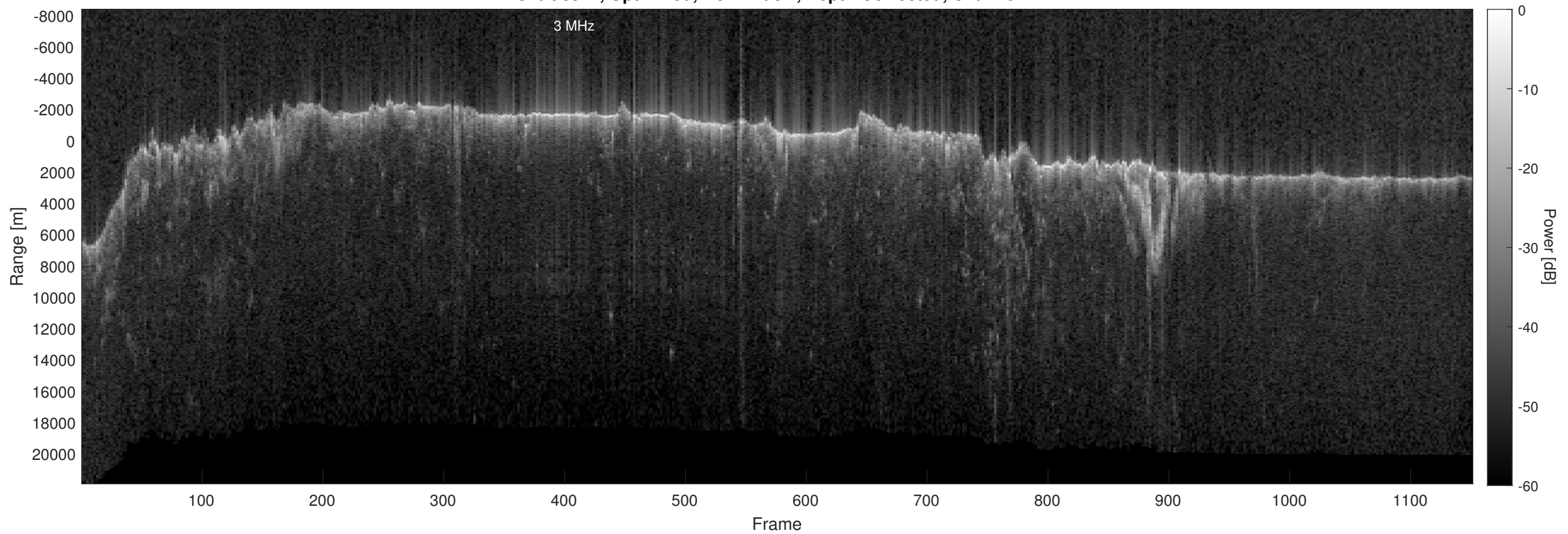
Orbit 3972, Optimized, No Window, Depth-Corrected, Channel 2
