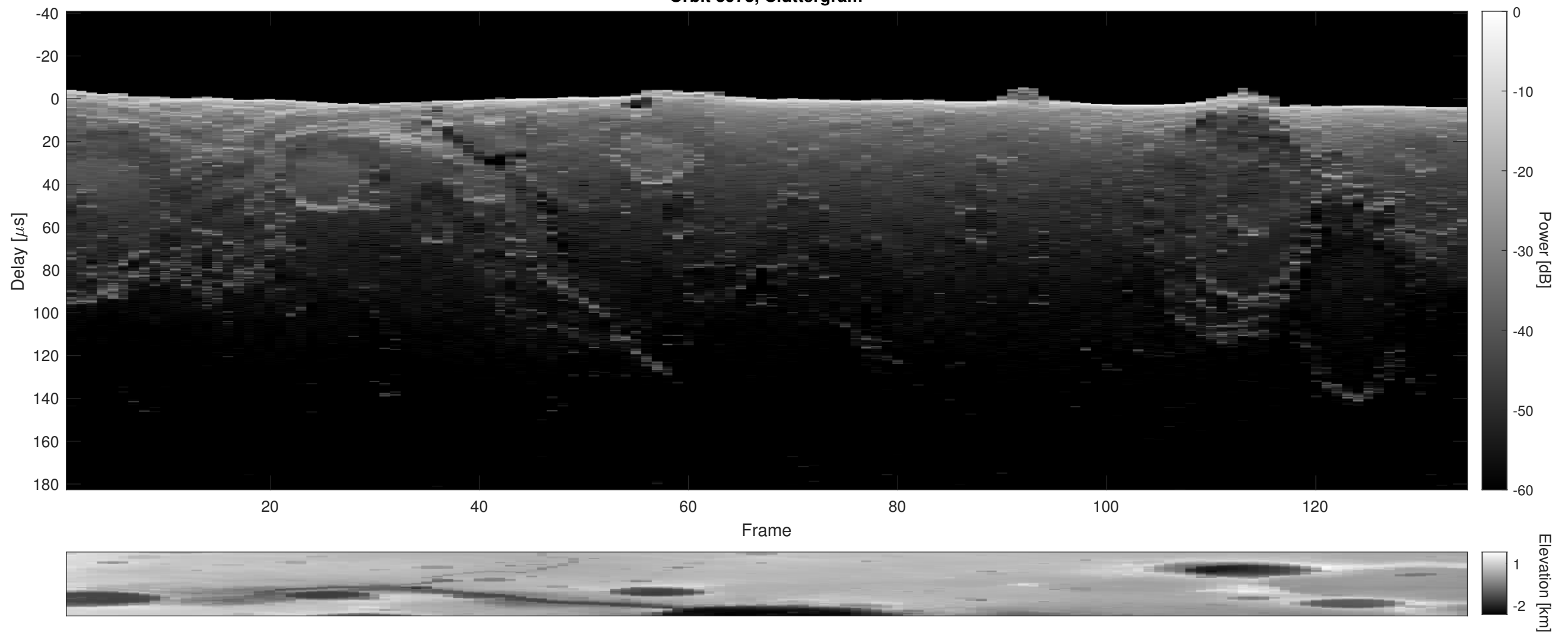
Orbit 3973, Cluttergram
