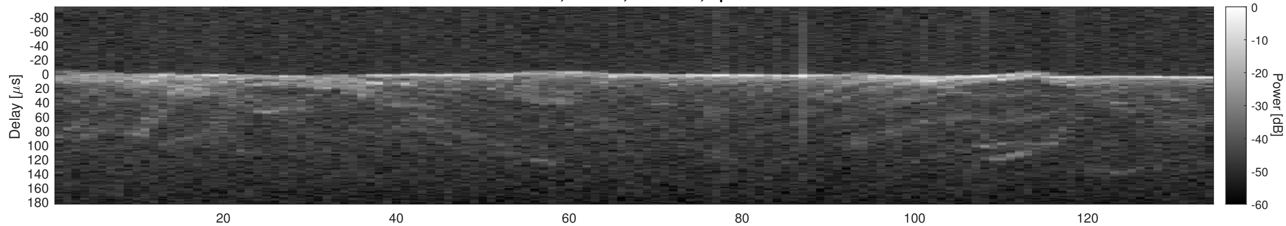
Orbit 3973, Cluttergram
