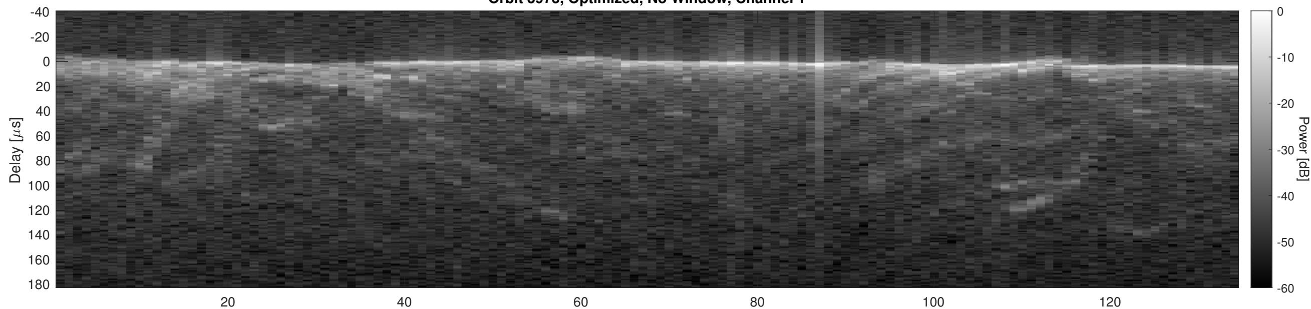
Orbit 3973, Optimized, No Window, Channel 2
