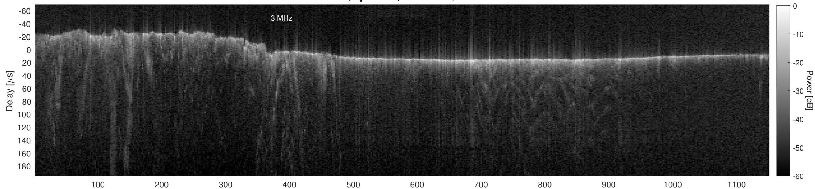
Orbit 3975, Cluttergram
