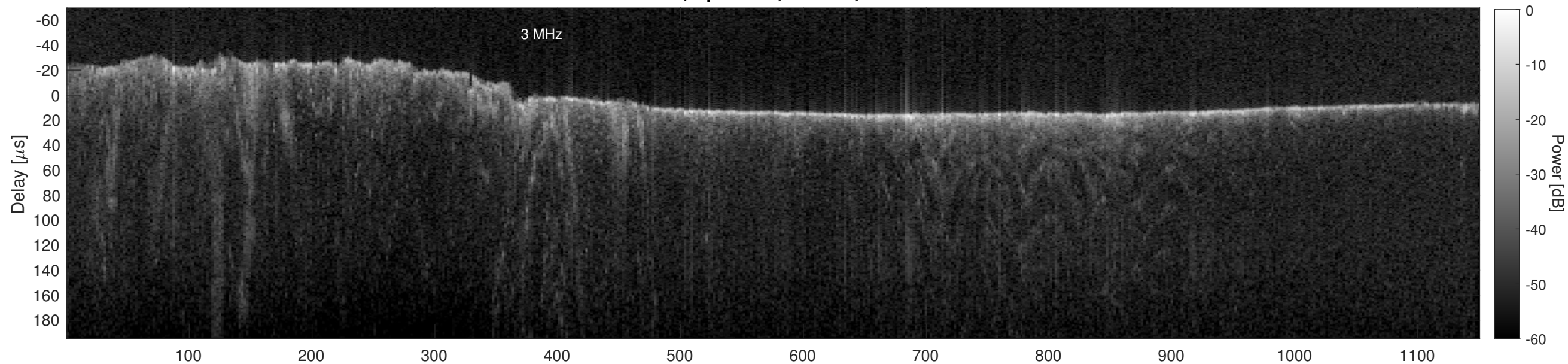
Orbit 3975, Cluttergram
