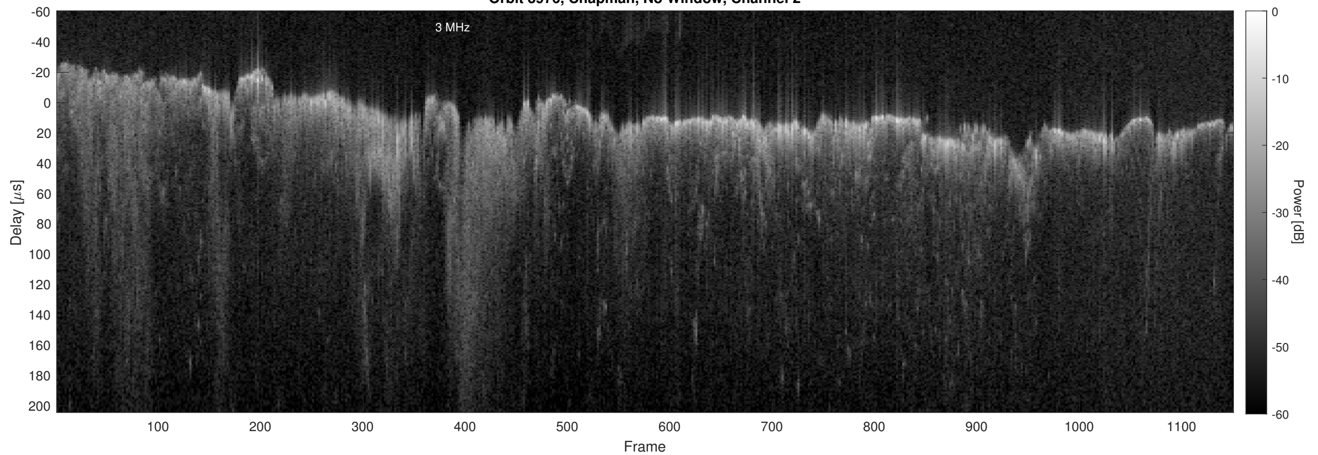
Orbit 3976, Chapman, No Window, Channel 2
