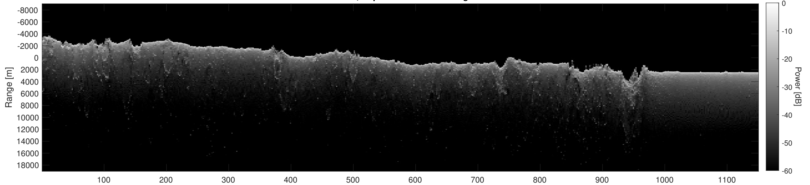
Orbit 3976, Depth-Corrected Cluttergram
