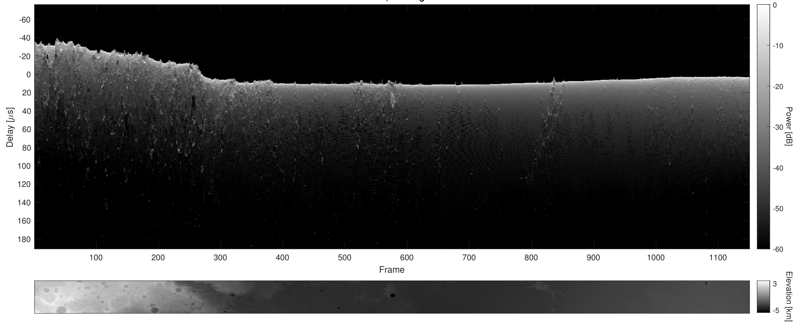
Orbit 3978, Cluttergram
