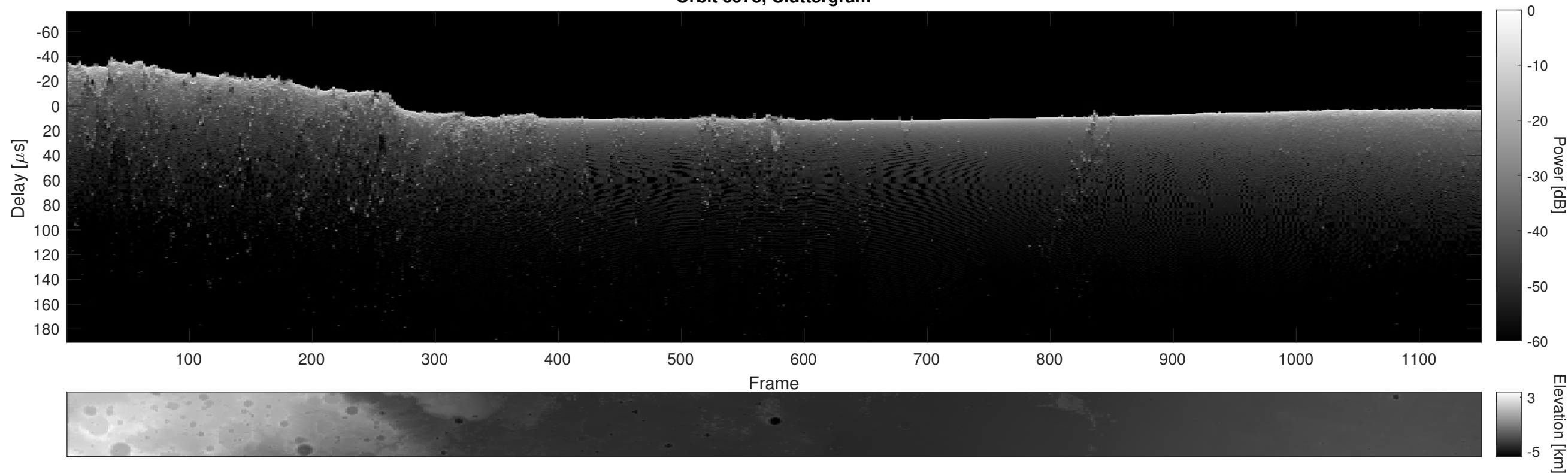
Orbit 3978, Cluttergram
