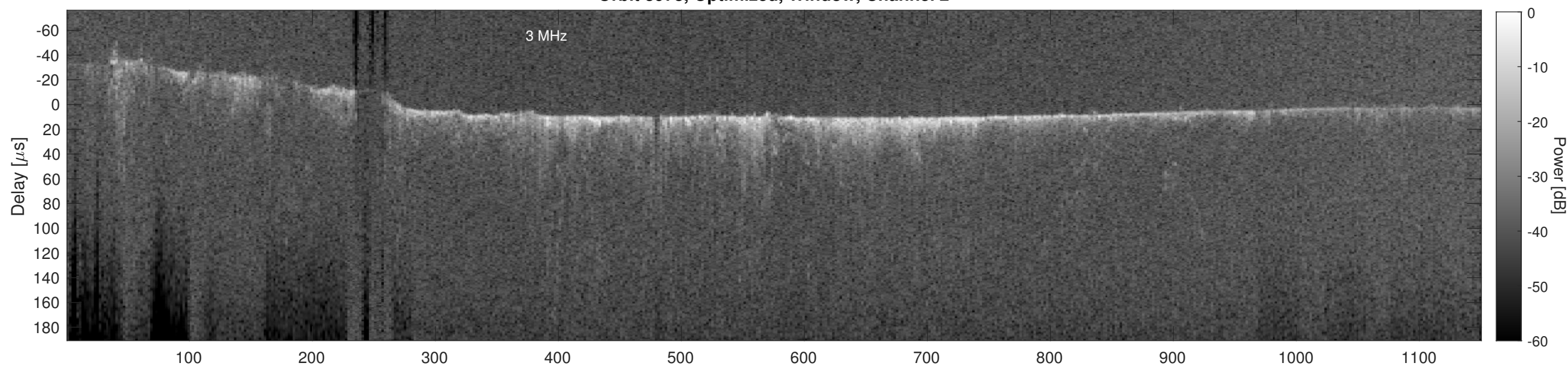
Orbit 3978, Cluttergram
