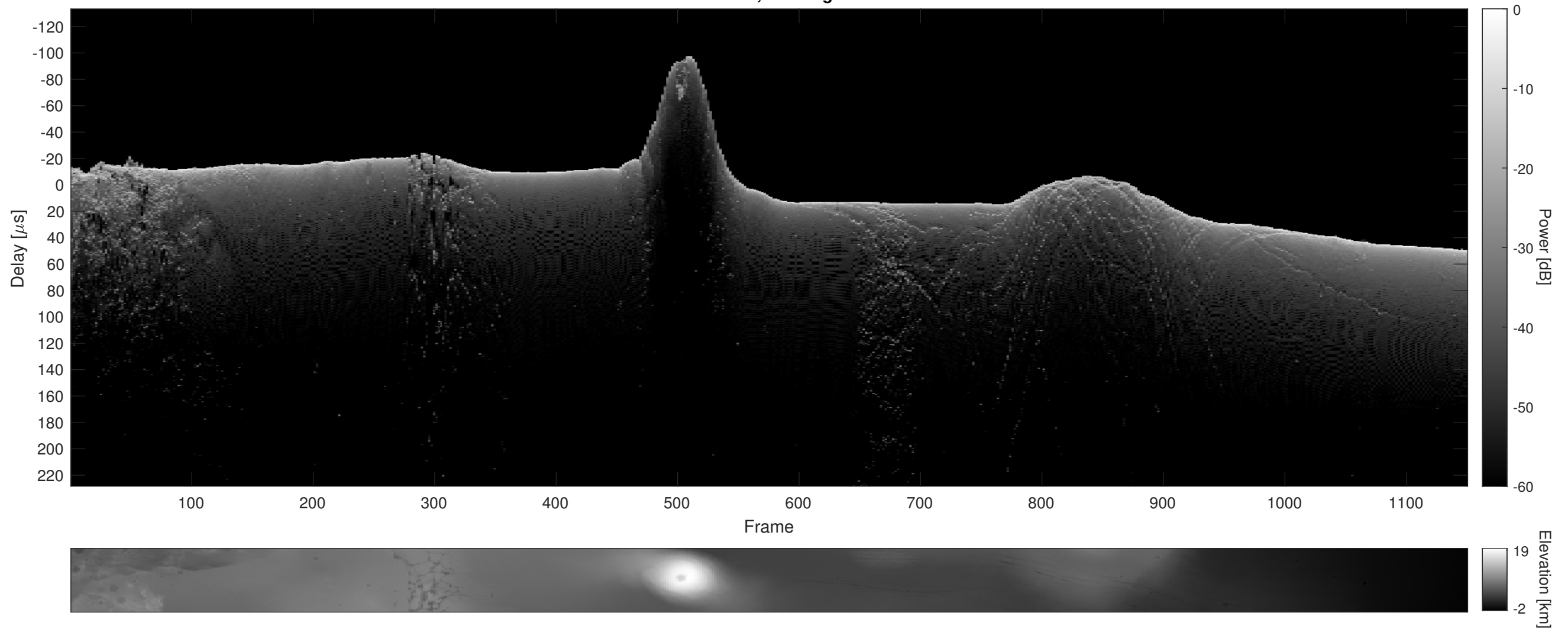
Orbit 3981, Cluttergram
