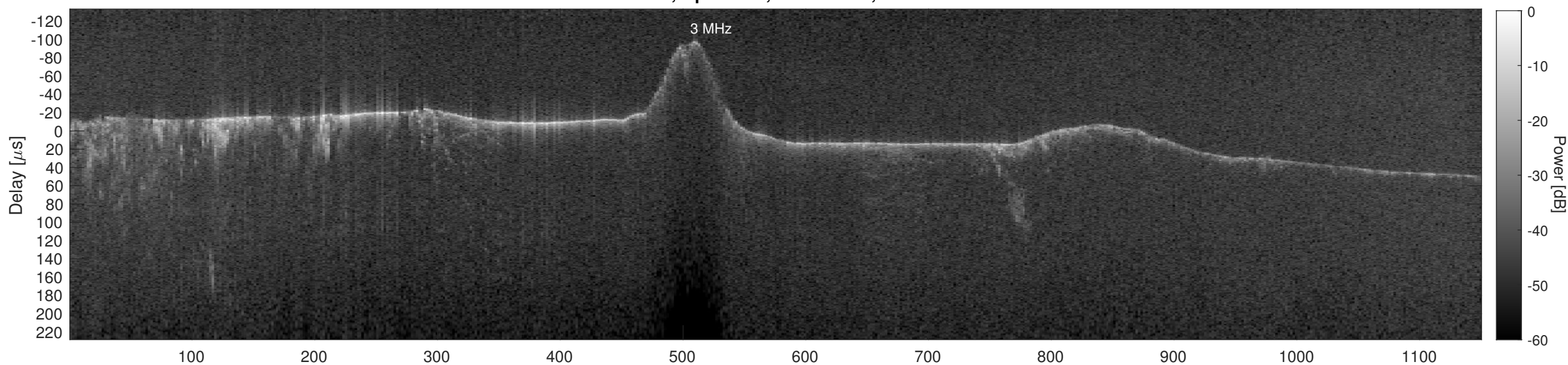
Orbit 3981, Cluttergram
