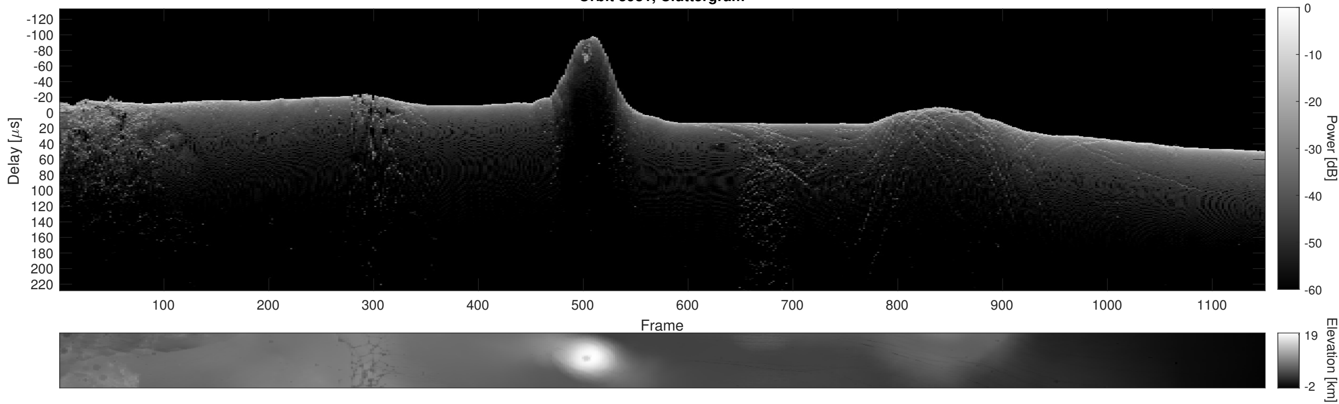
Orbit 3981, Cluttergram
