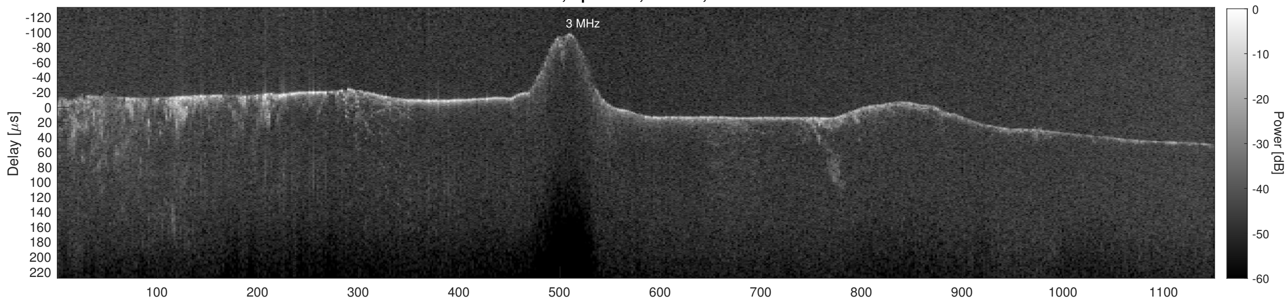
Orbit 3981, Cluttergram
