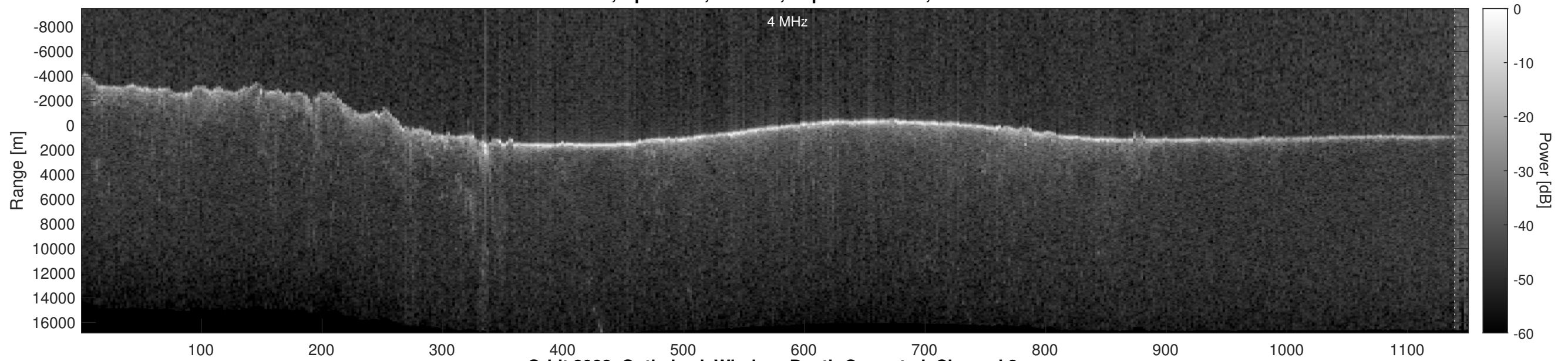
Orbit 3982, Optimized, Window, Depth-Corrected, Channel 2
