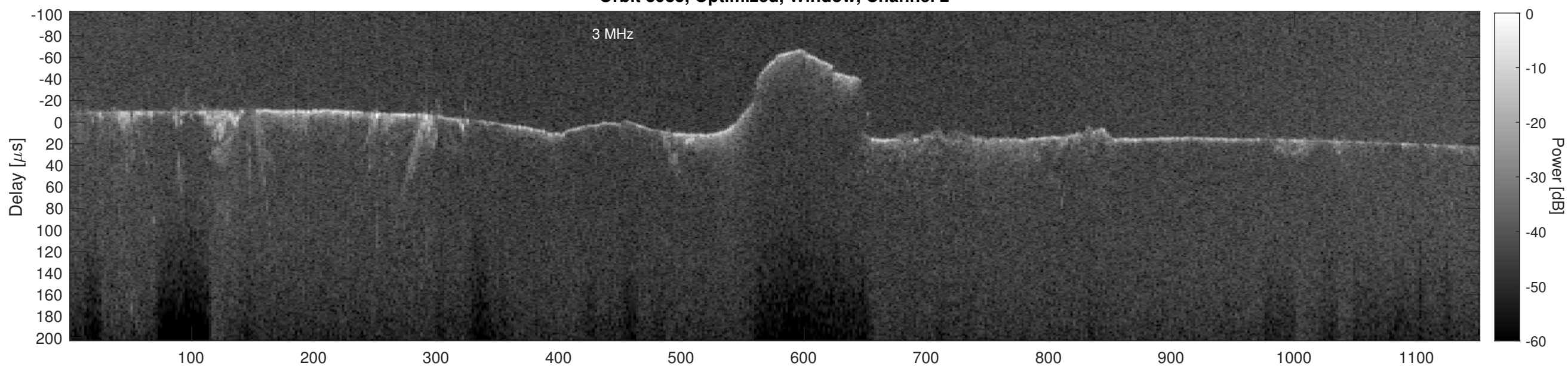
Orbit 3985, Cluttergram
