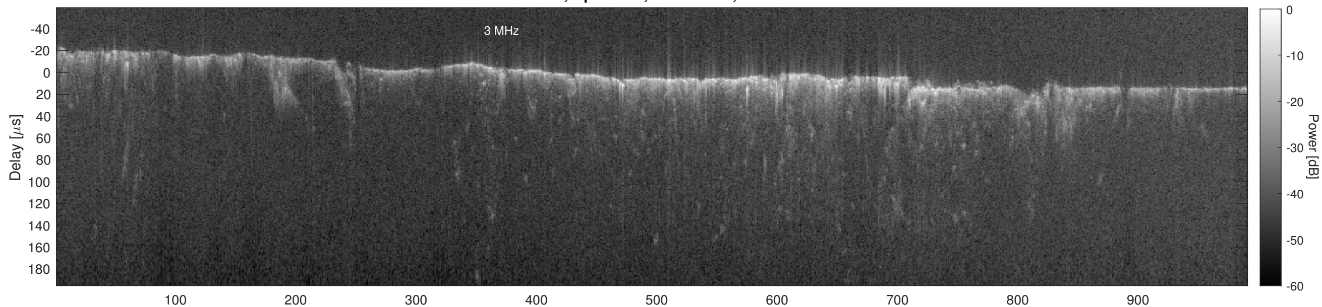
Orbit 3987, Cluttergram
