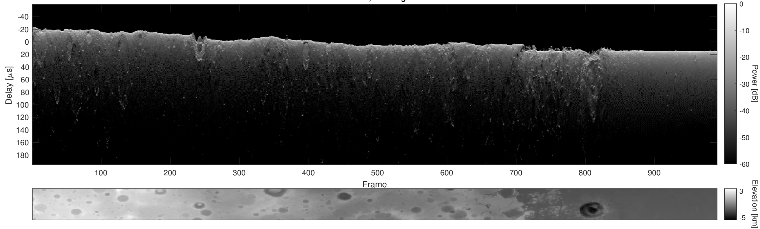
Orbit 3987, Cluttergram
