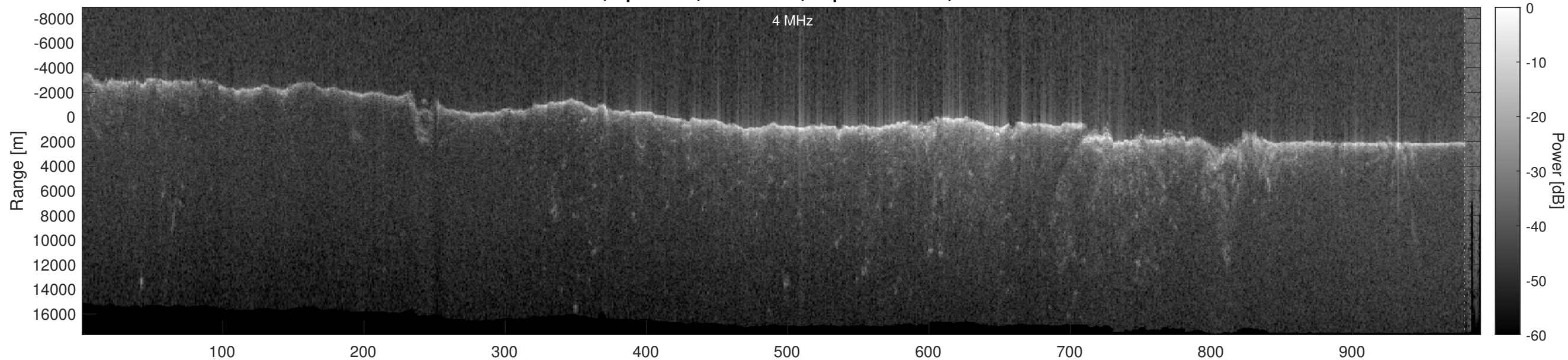
Orbit 3987, Optimized, No Window, Depth-Corrected, Channel 2
