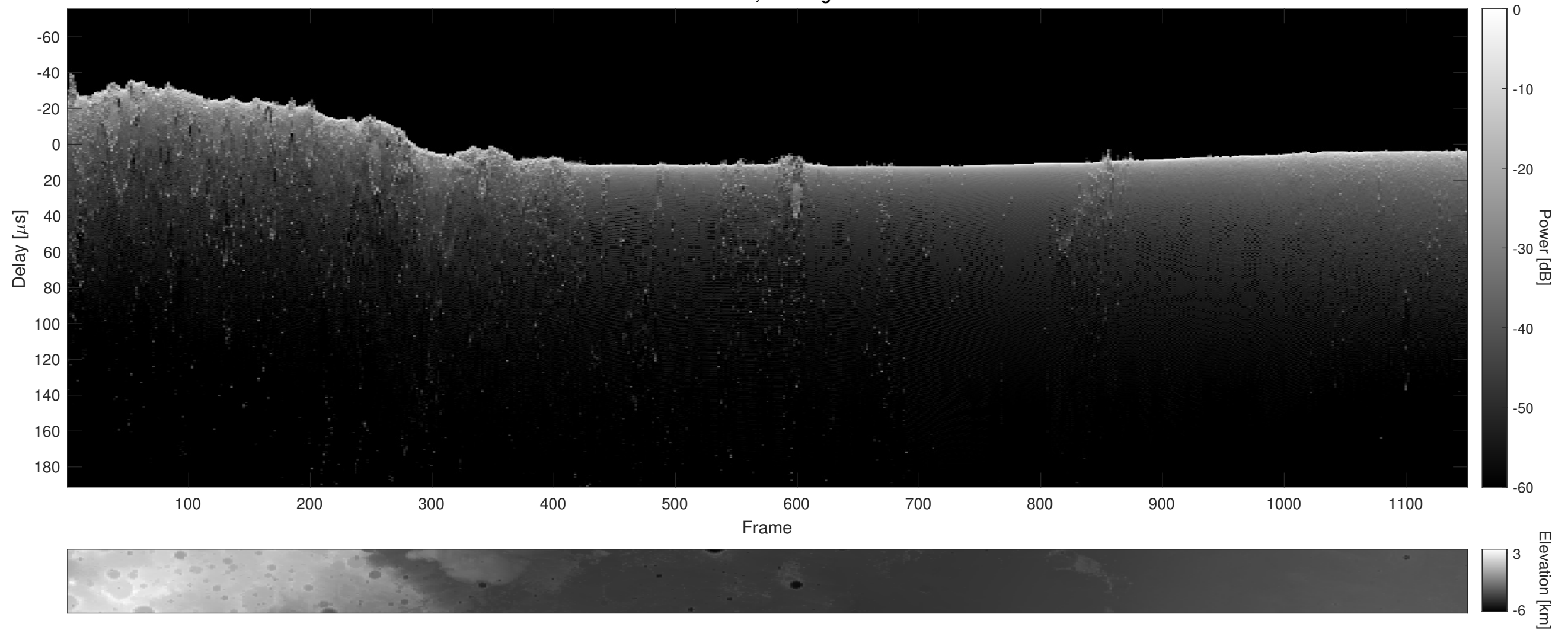
Orbit 3989, Cluttergram
