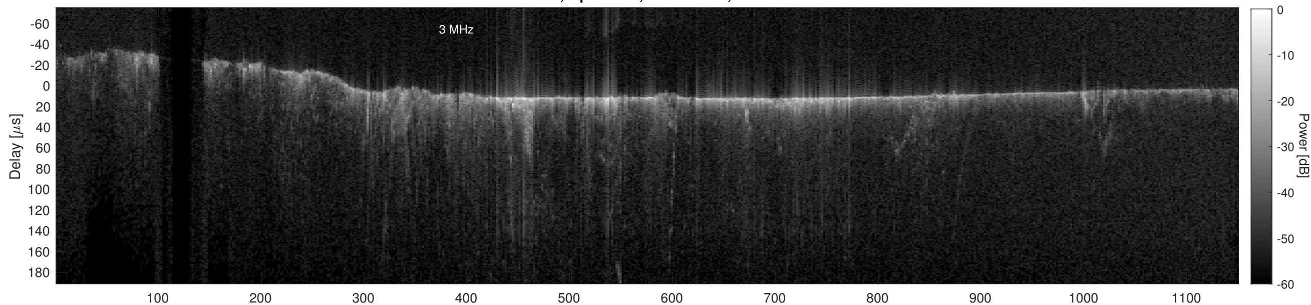
Orbit 3989, Cluttergram
