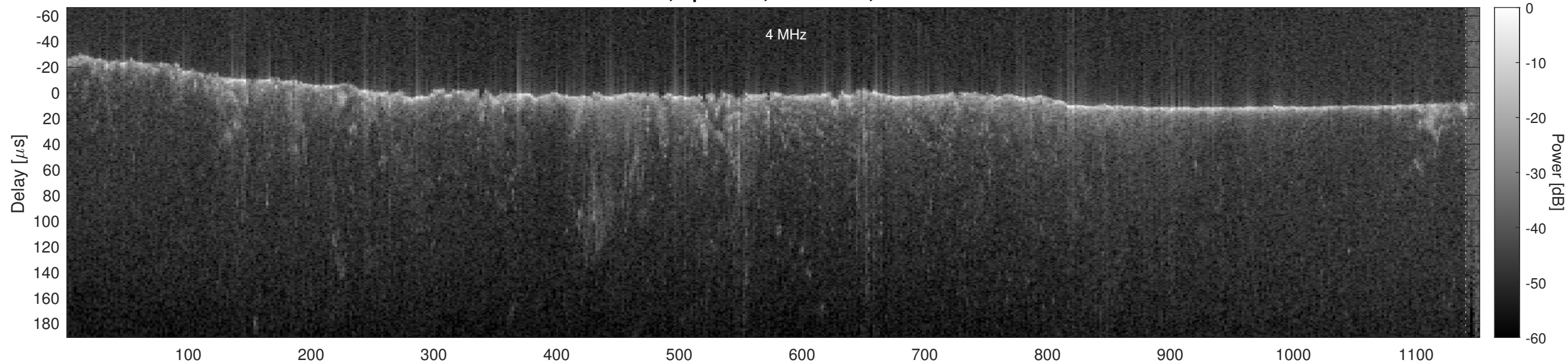
Orbit 3991, Optimized, No Window, Channel 2
