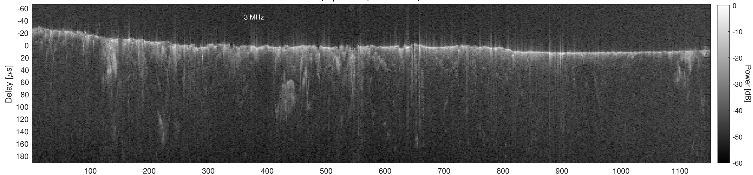
Orbit 3991, Cluttergram
