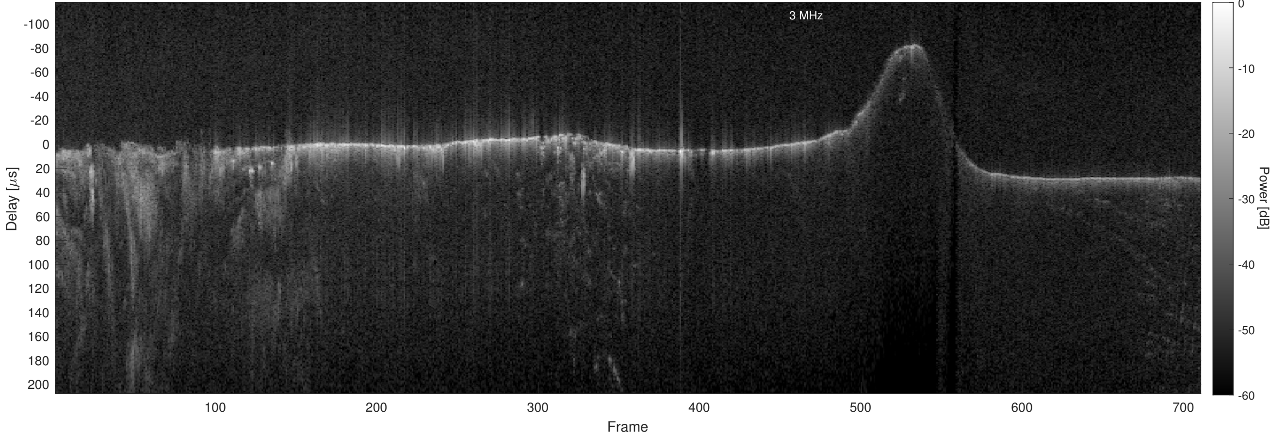
Orbit 3992, Optimized, No Window, Channel 2
