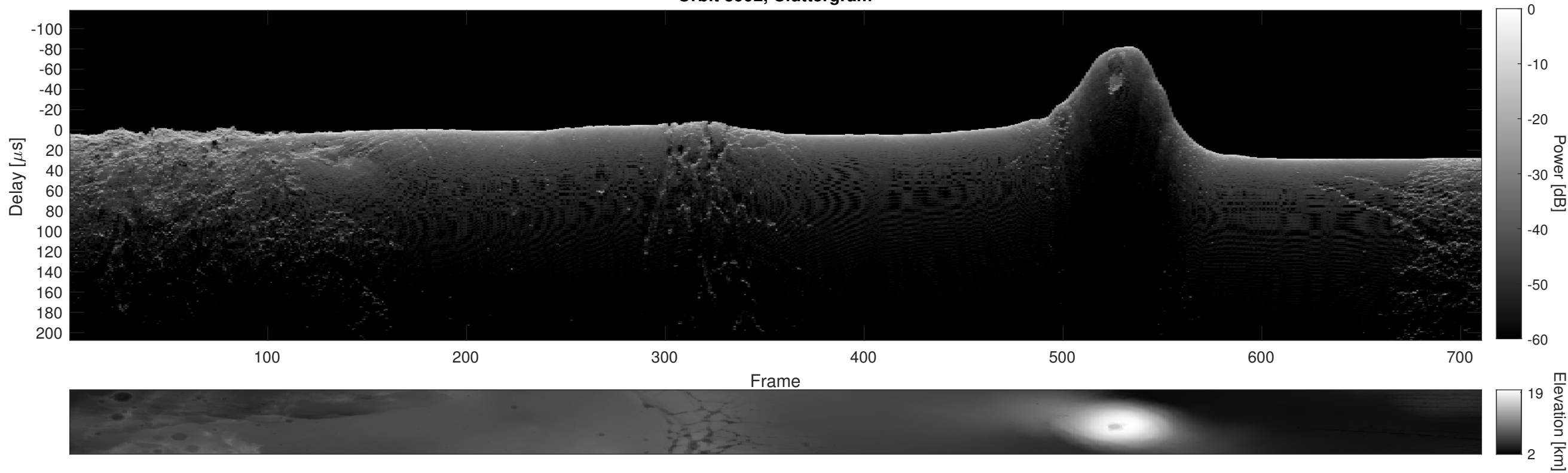
Orbit 3992, Cluttergram
