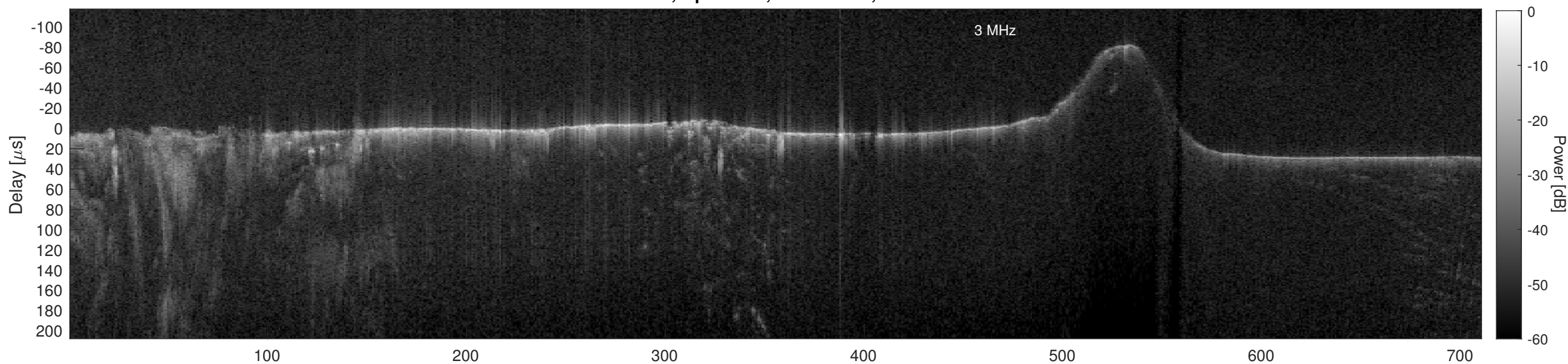
Orbit 3992, Cluttergram
