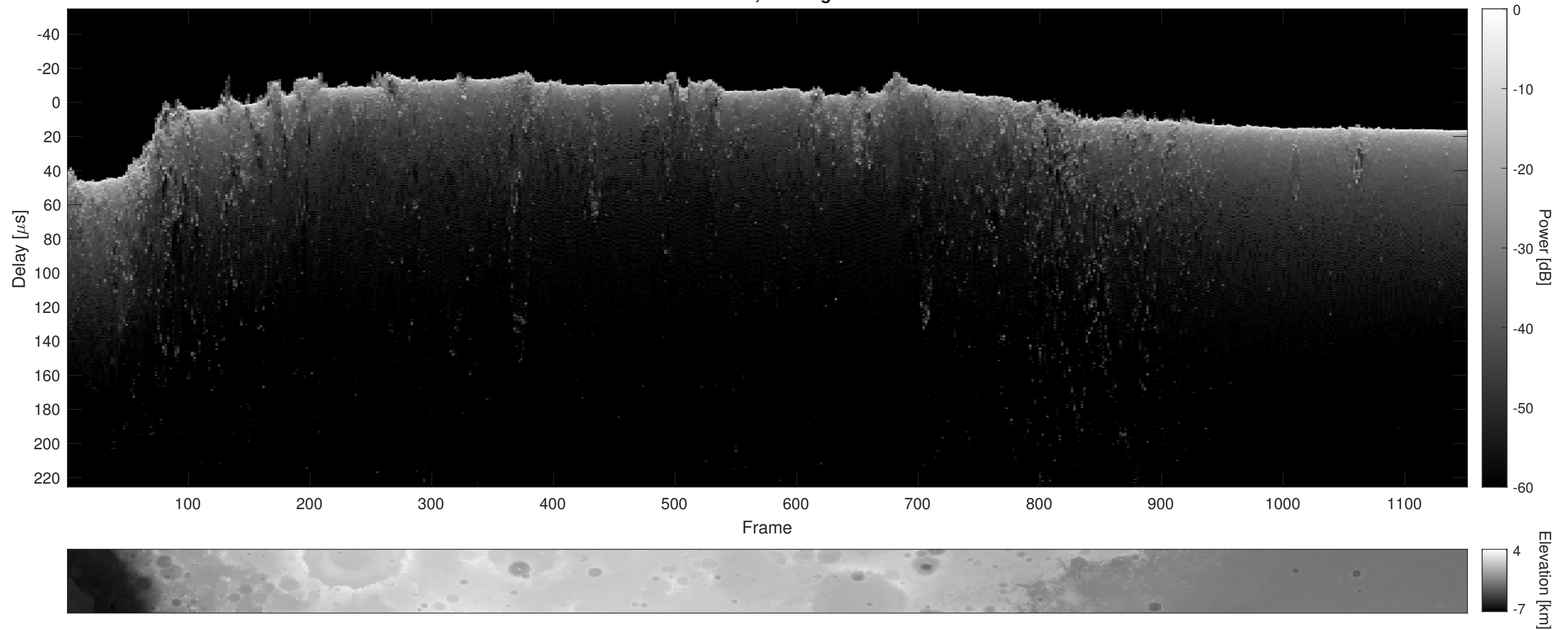
Orbit 3994, Cluttergram
