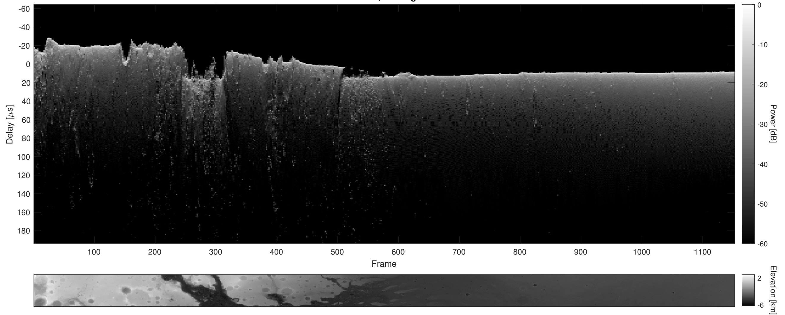
Orbit 3995, Cluttergram
