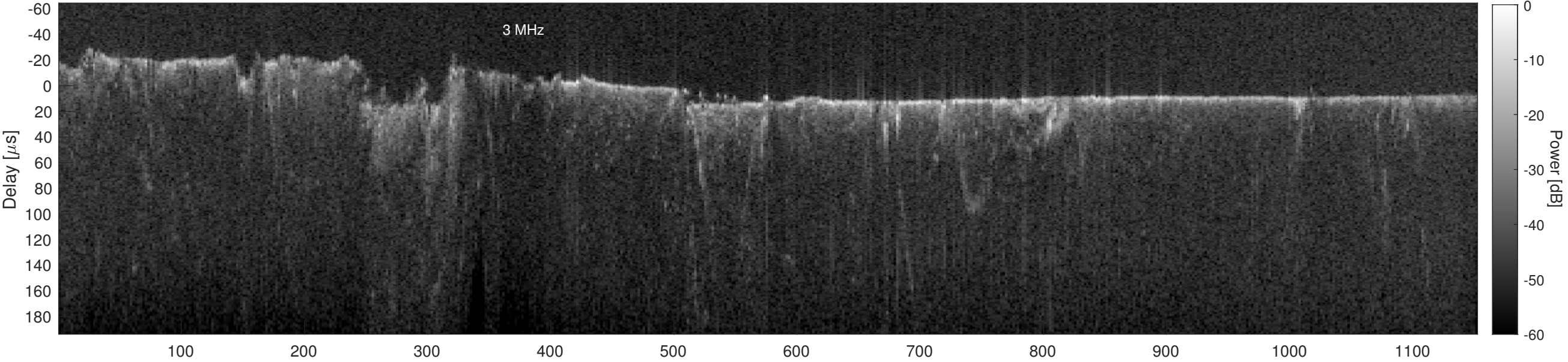
Orbit 3995, Cluttergram
