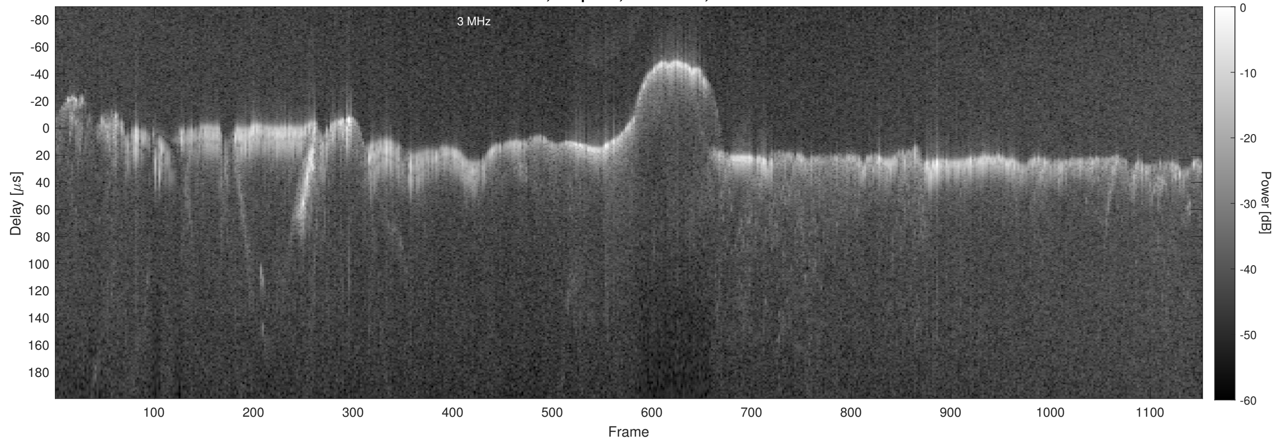
Orbit 3996, Chapman, No Window, Channel 2
