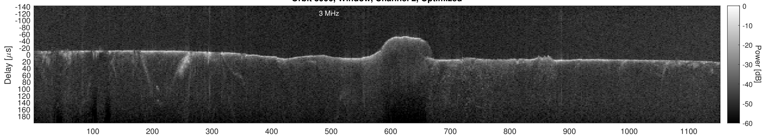
Orbit 3996, Cluttergram
