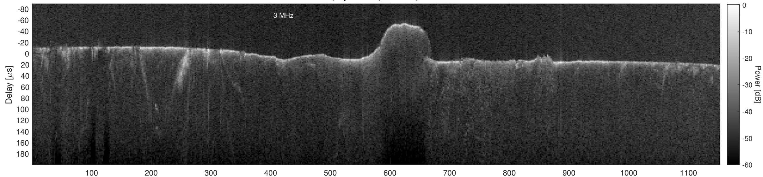
Orbit 3996, Cluttergram
