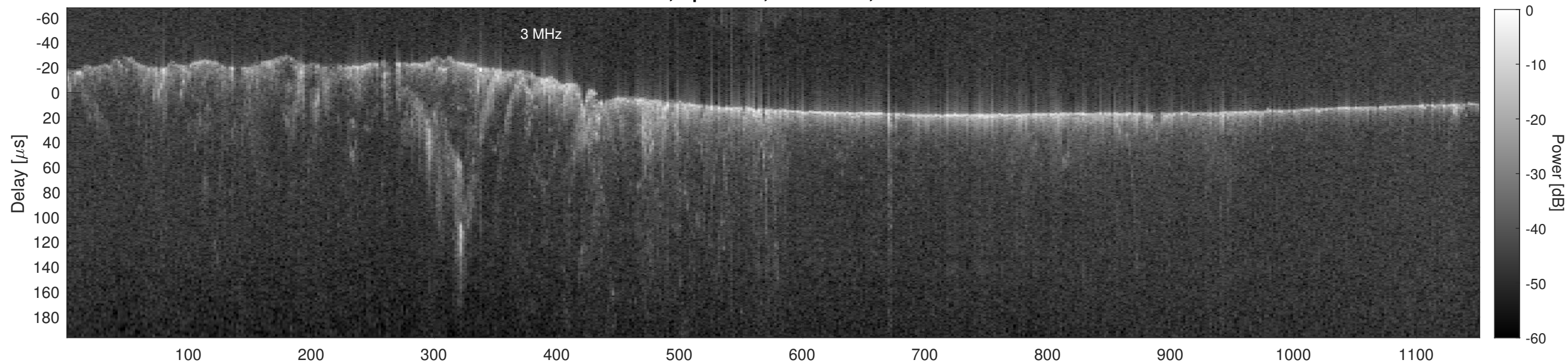
Orbit 3997, Cluttergram
