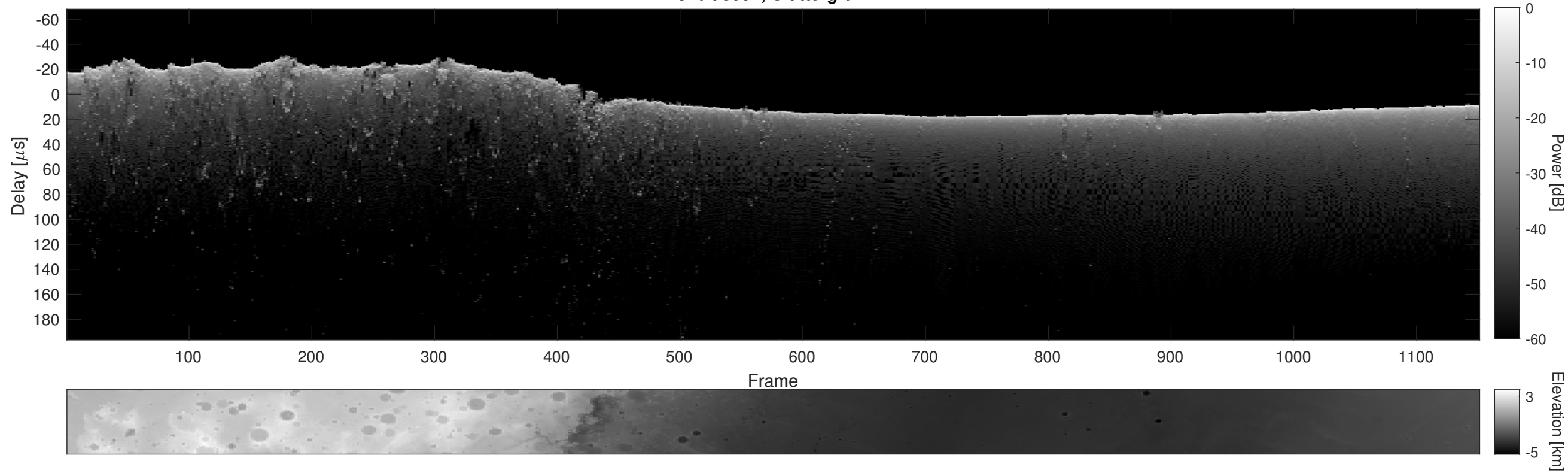
Orbit 3997, Cluttergram
