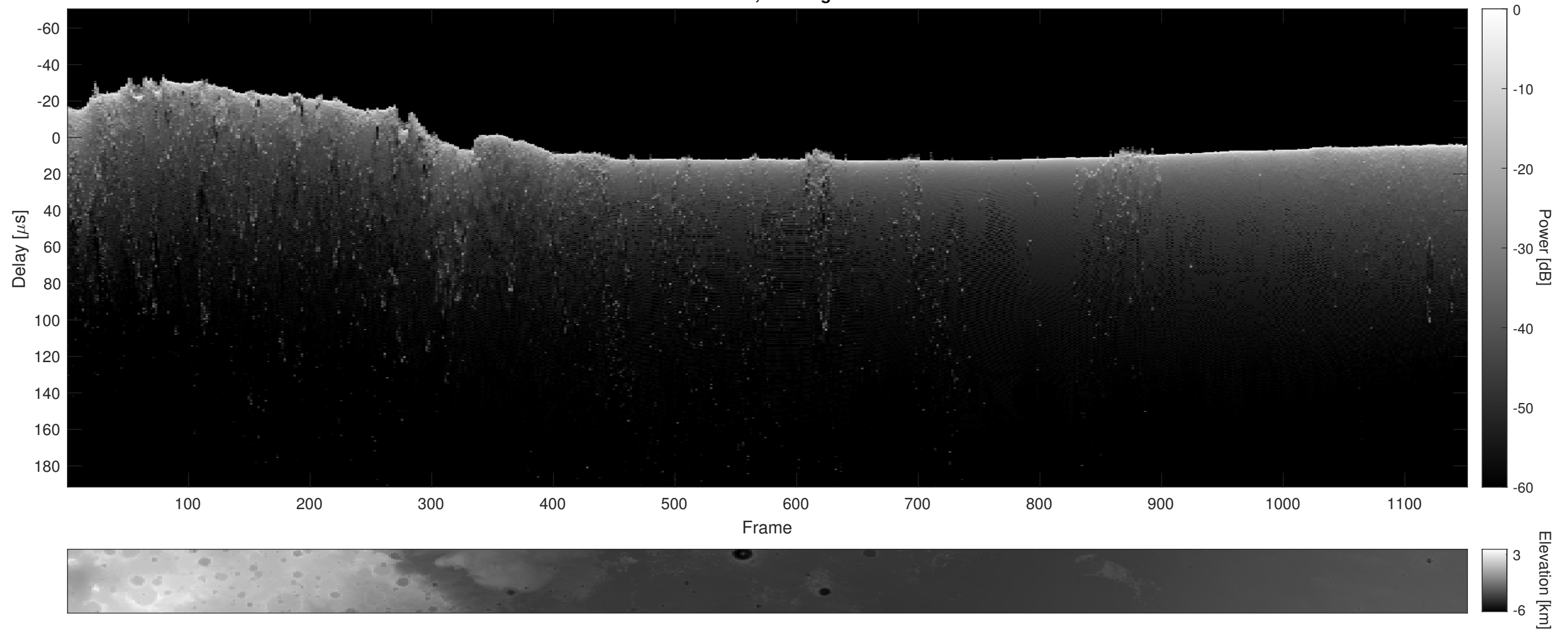
Orbit 4000, Cluttergram
