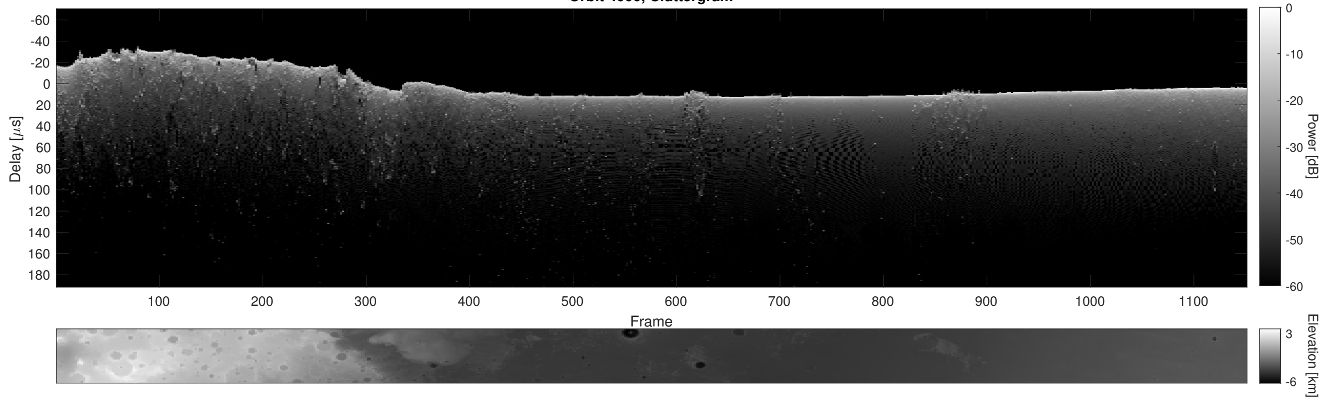
Orbit 4000, Cluttergram
