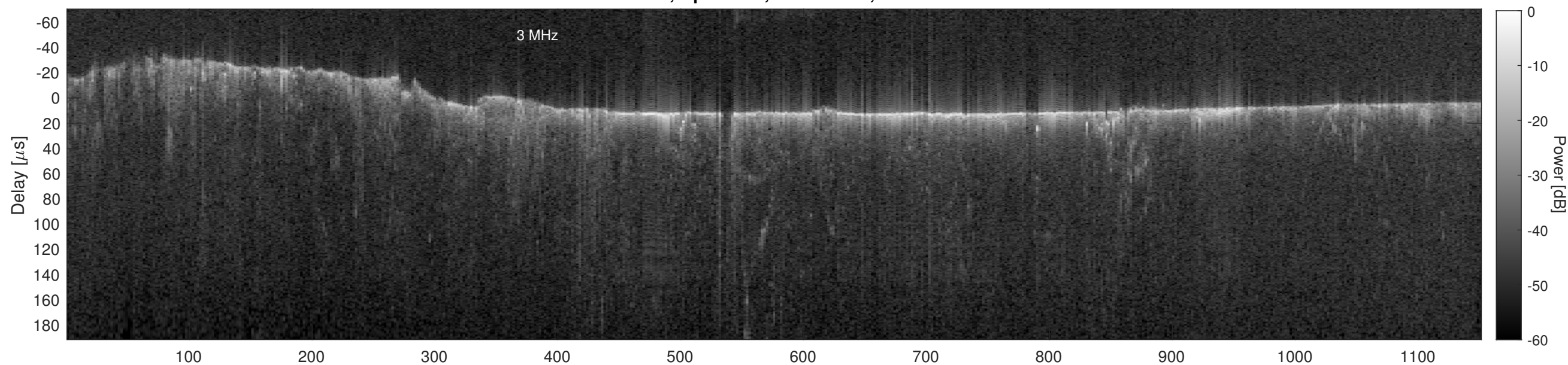
Orbit 4000, Cluttergram
