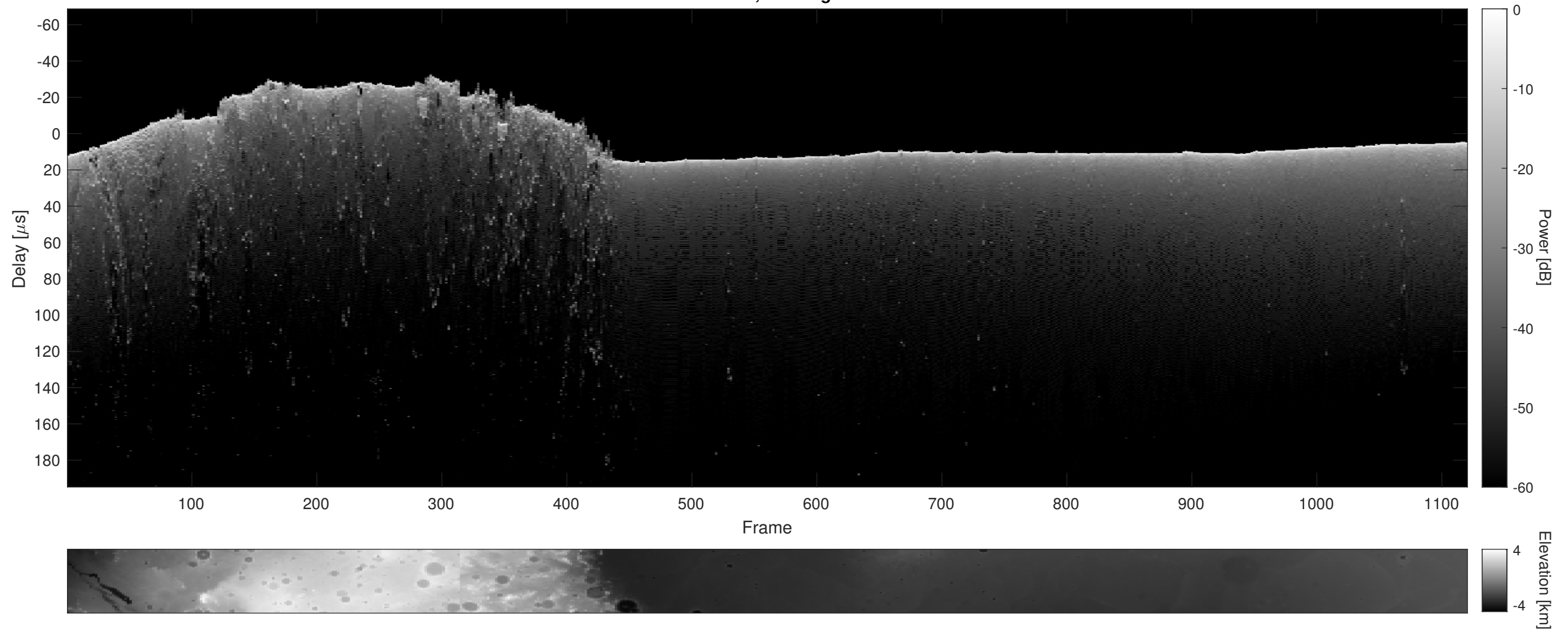
Orbit 4001, Cluttergram
