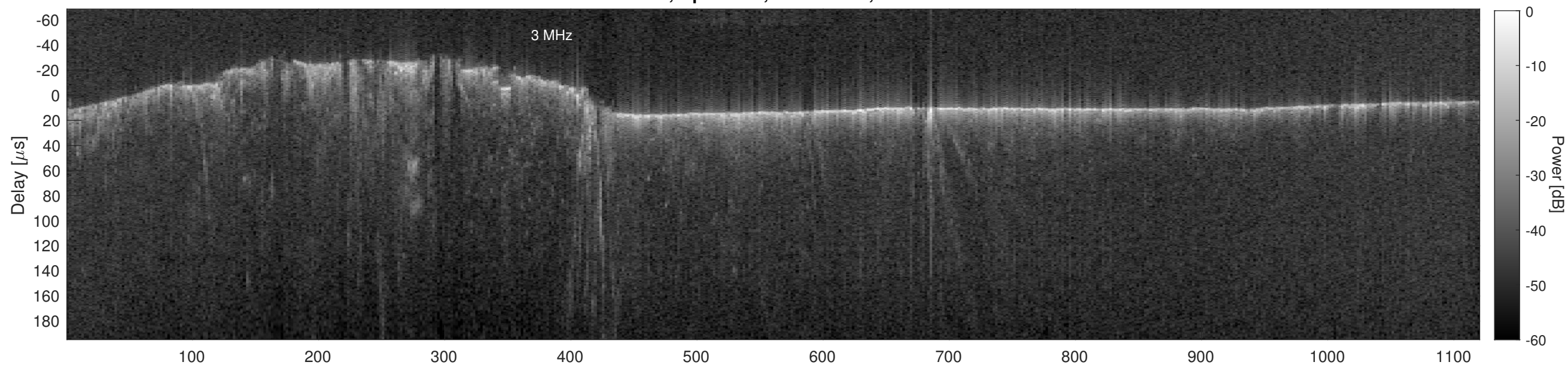
Orbit 4001, Cluttergram
