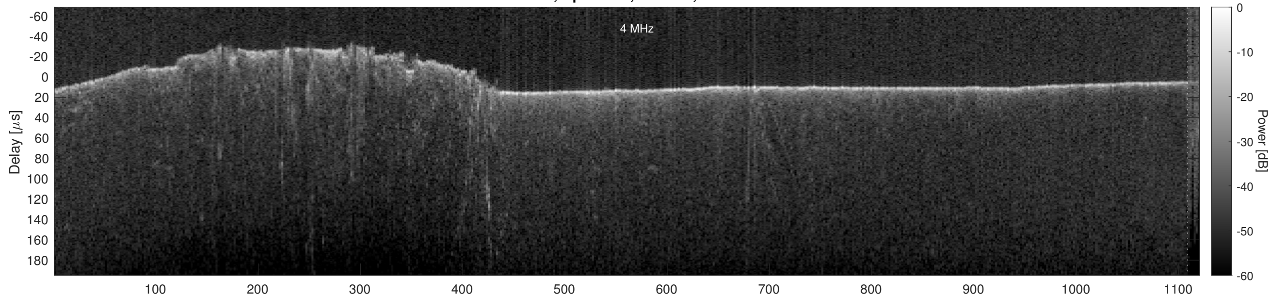
Orbit 4001, Optimized, Window, Channel 2
