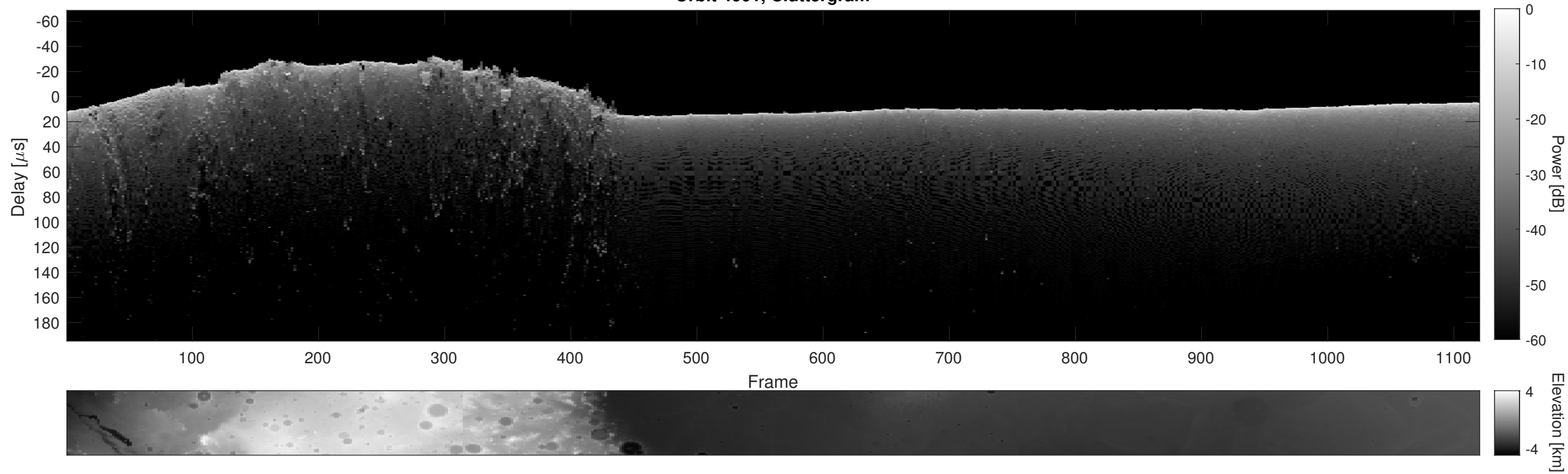
Orbit 4001, Cluttergram
