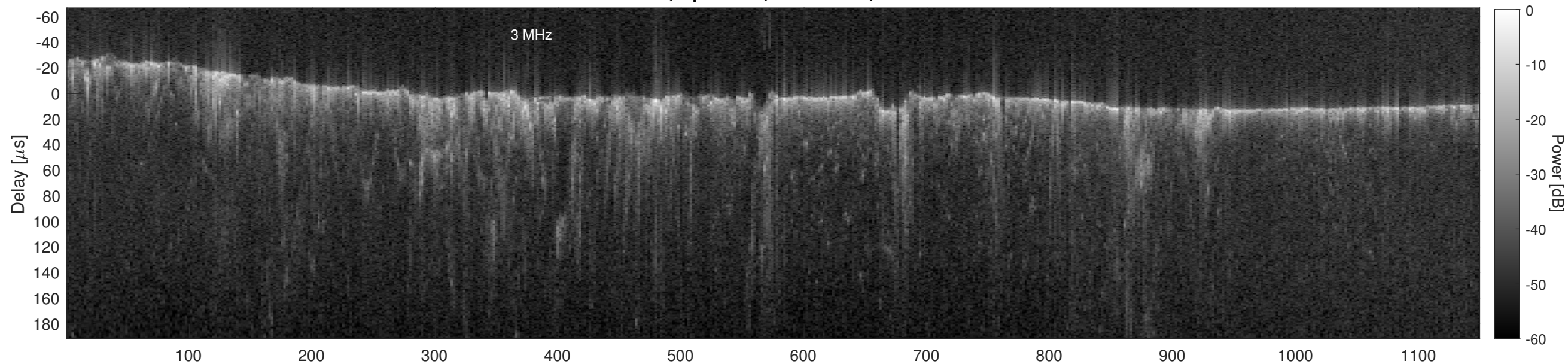
Orbit 4002, Cluttergram
