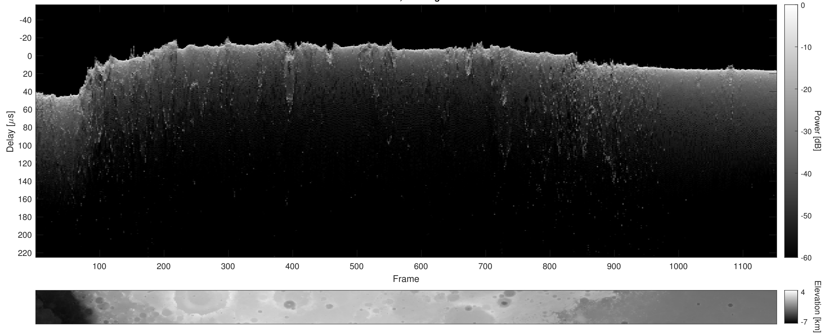
Orbit 4005, Cluttergram
