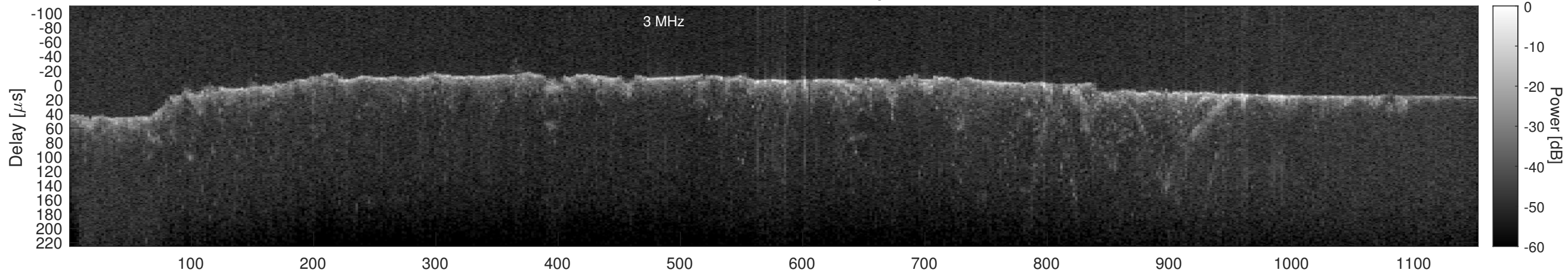
Orbit 4005, Cluttergram
