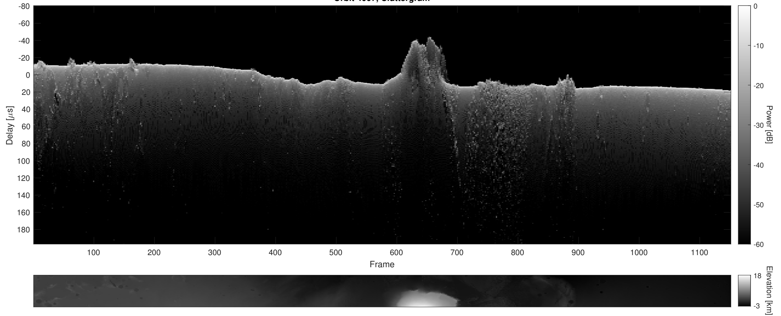
Orbit 4007, Cluttergram
