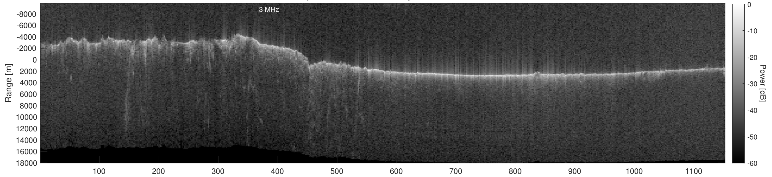
Orbit 4008, Depth-Corrected Cluttergram
