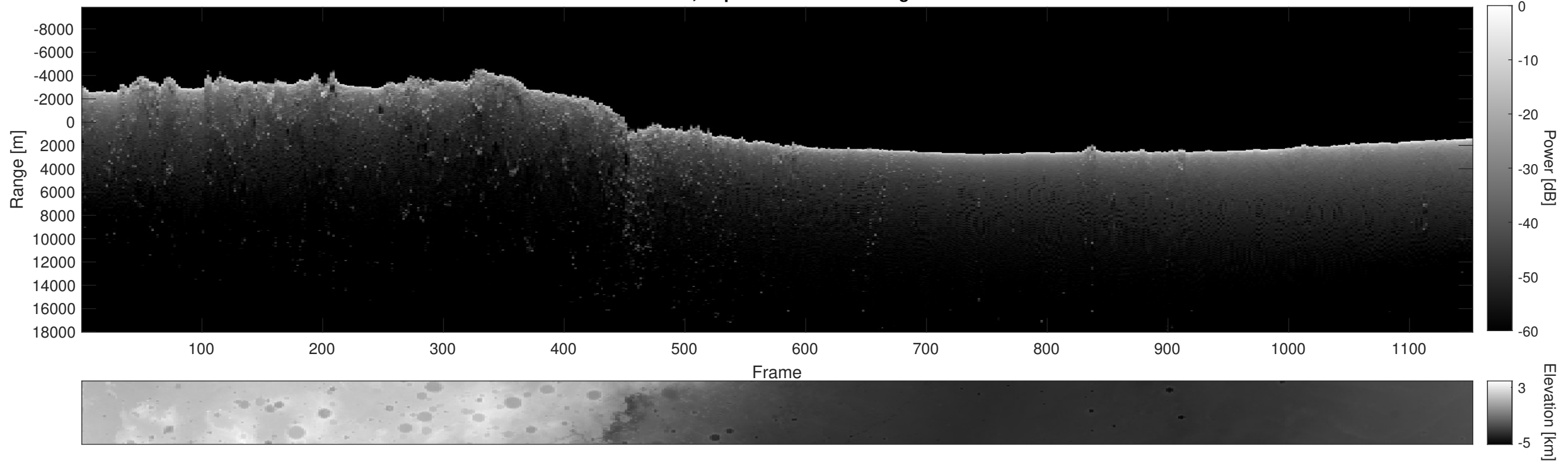
Orbit 4008, Depth-Corrected Cluttergram
