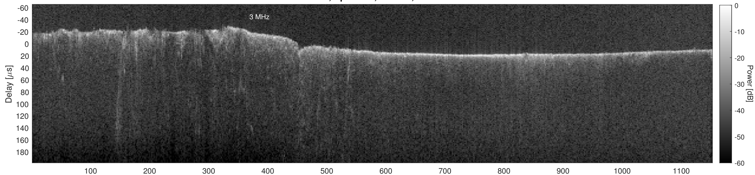
Orbit 4008, Cluttergram
