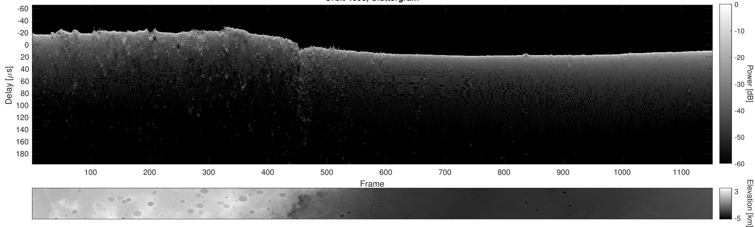
Orbit 4008, Cluttergram
