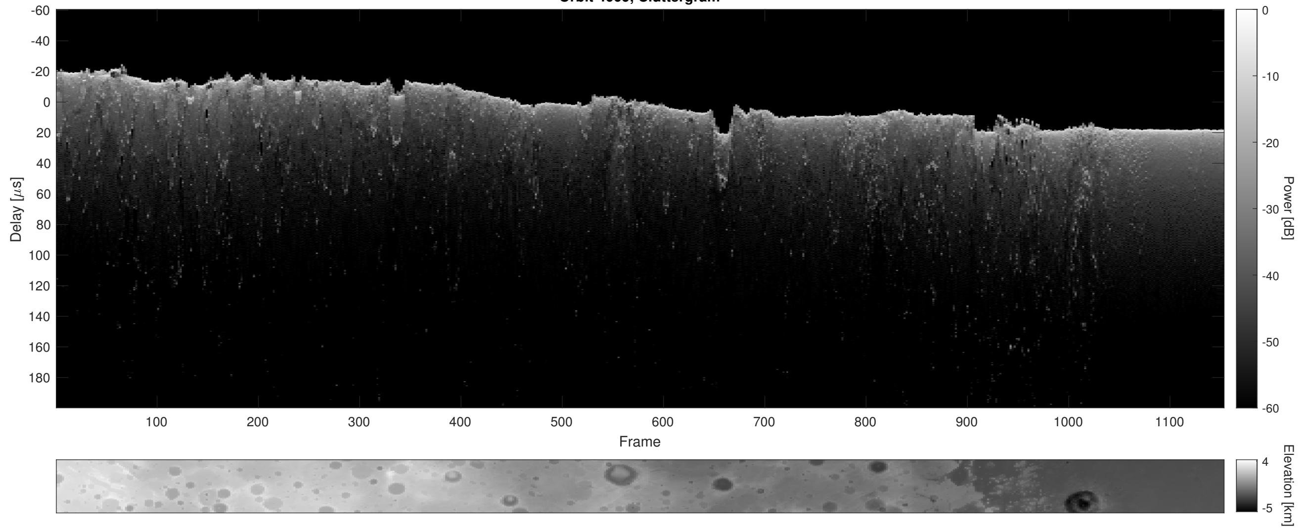
Orbit 4009, Cluttergram
