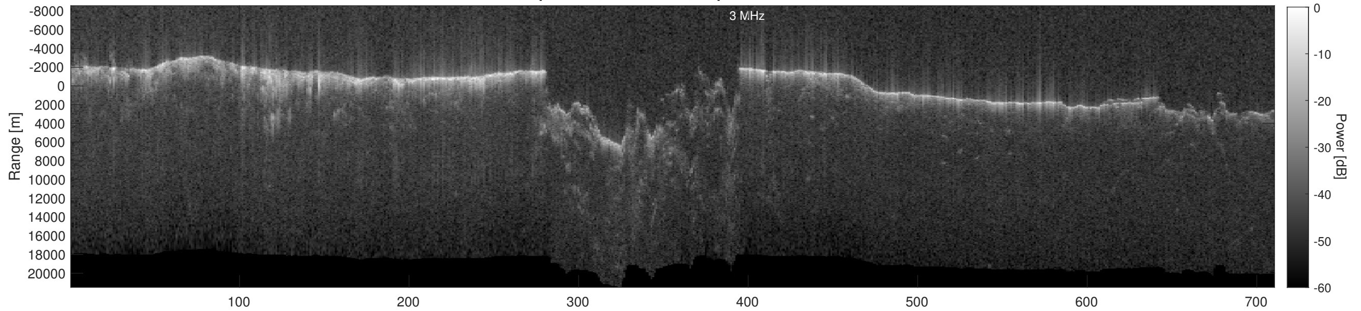
Orbit 4010, Depth-Corrected Cluttergram
