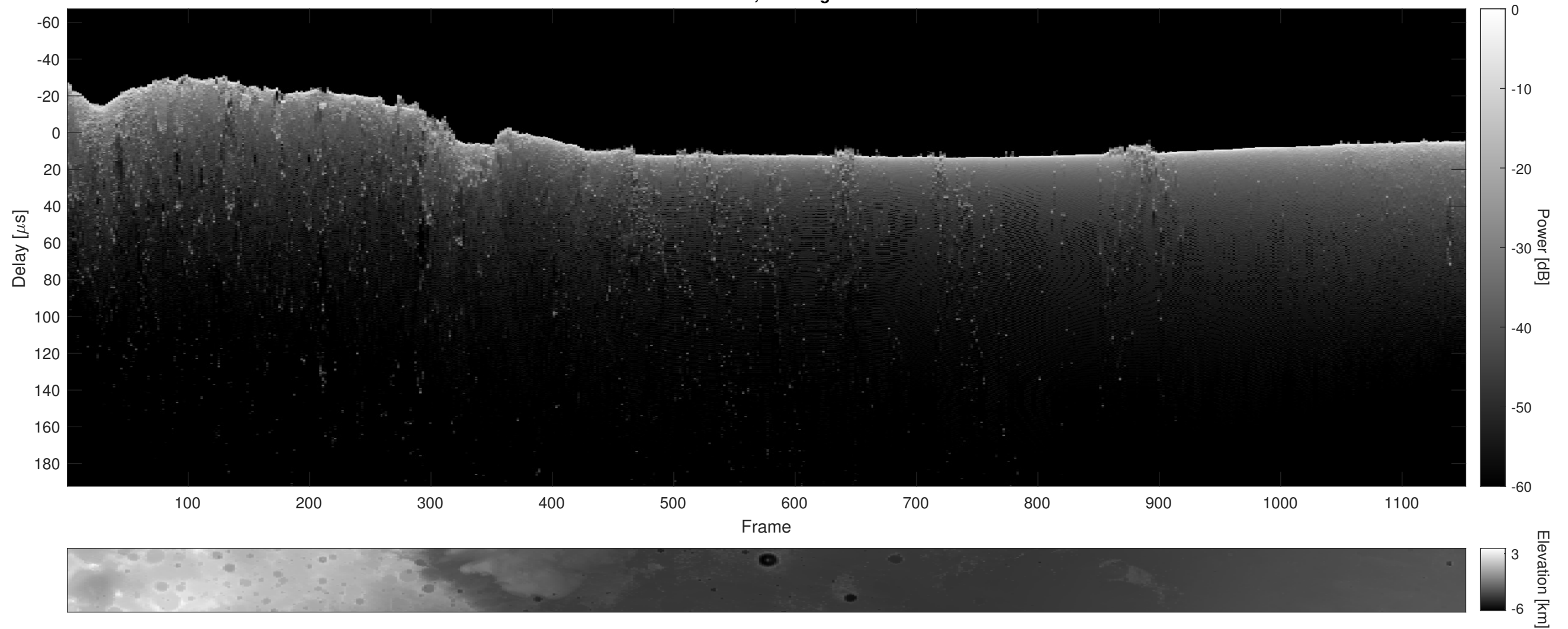
Orbit 4011, Cluttergram
