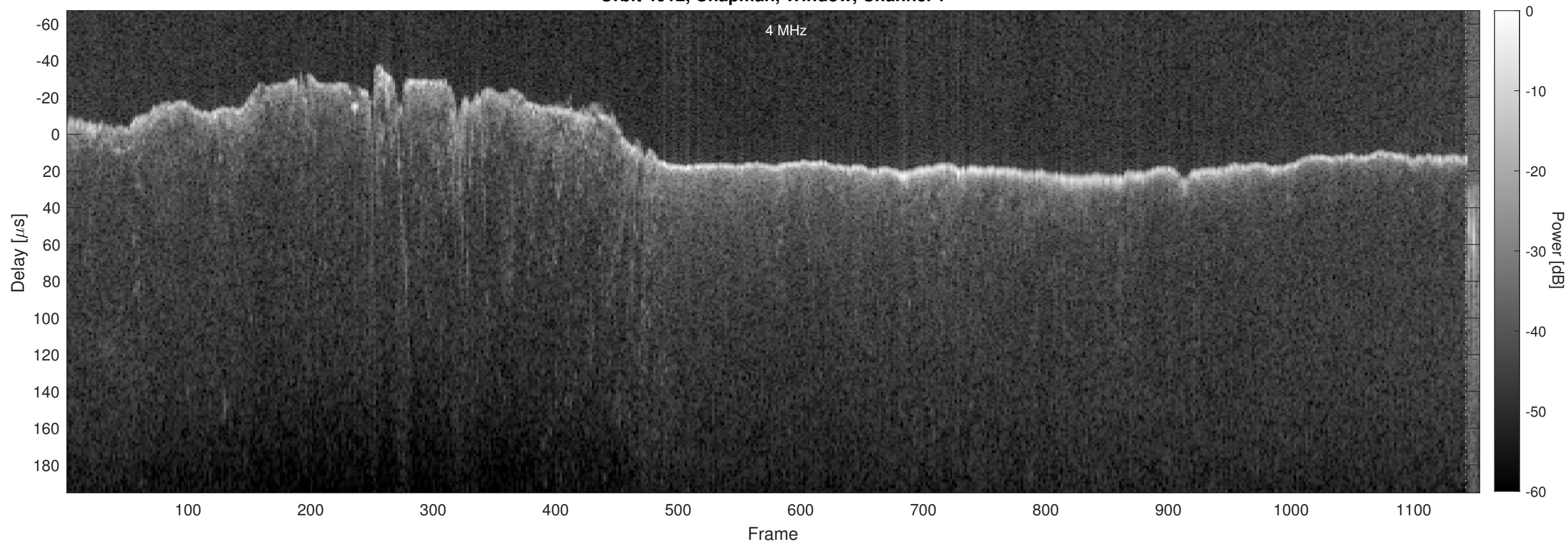
Orbit 4012, Chapman, Window, Channel 2
