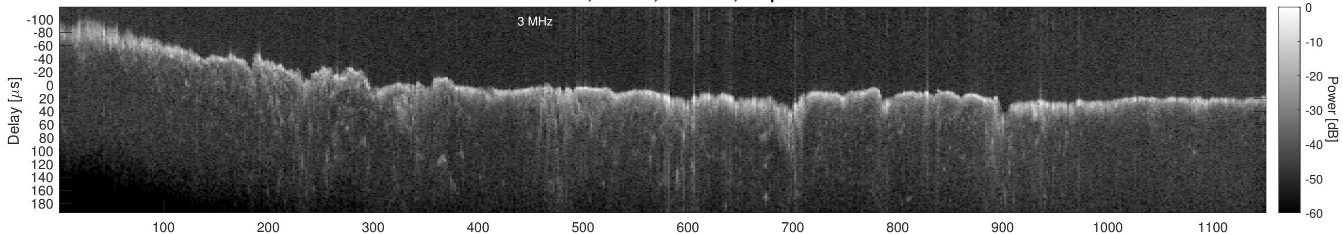
Orbit 4013, Window, Channel 2, Optimized
