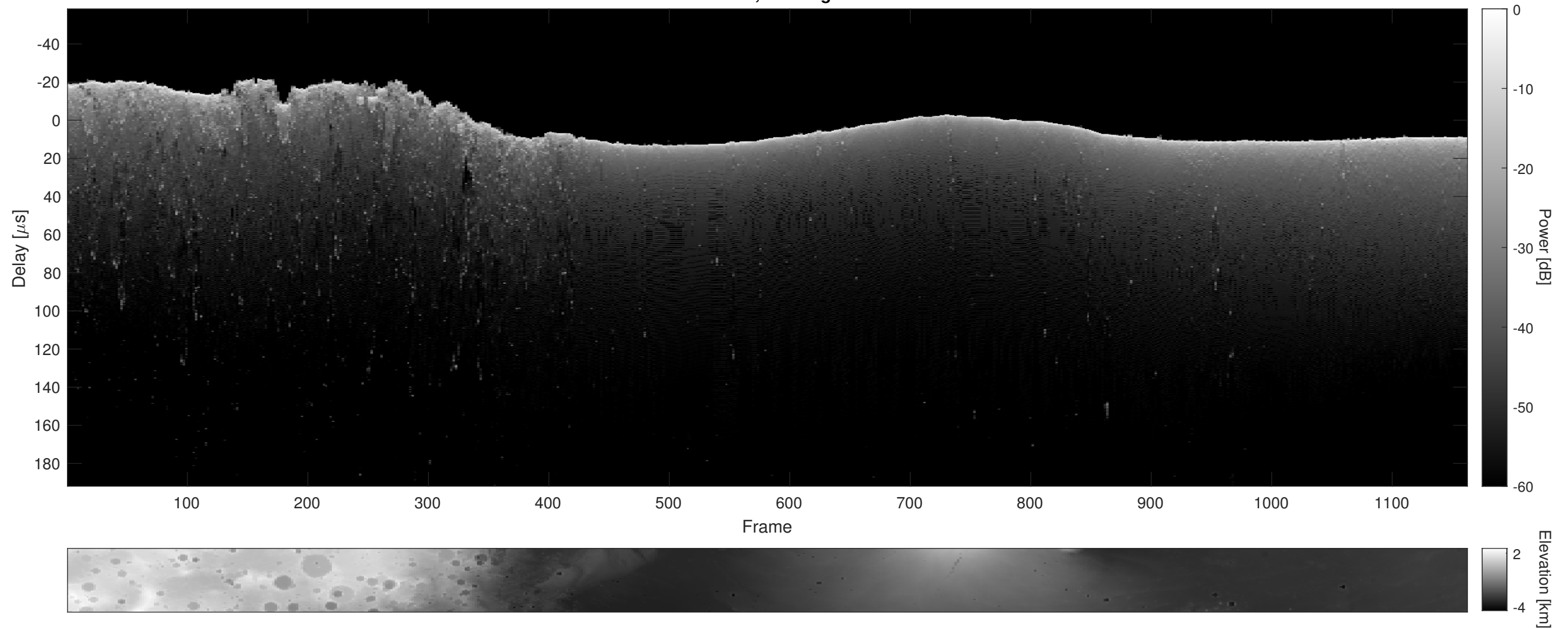
Orbit 4015, Cluttergram
