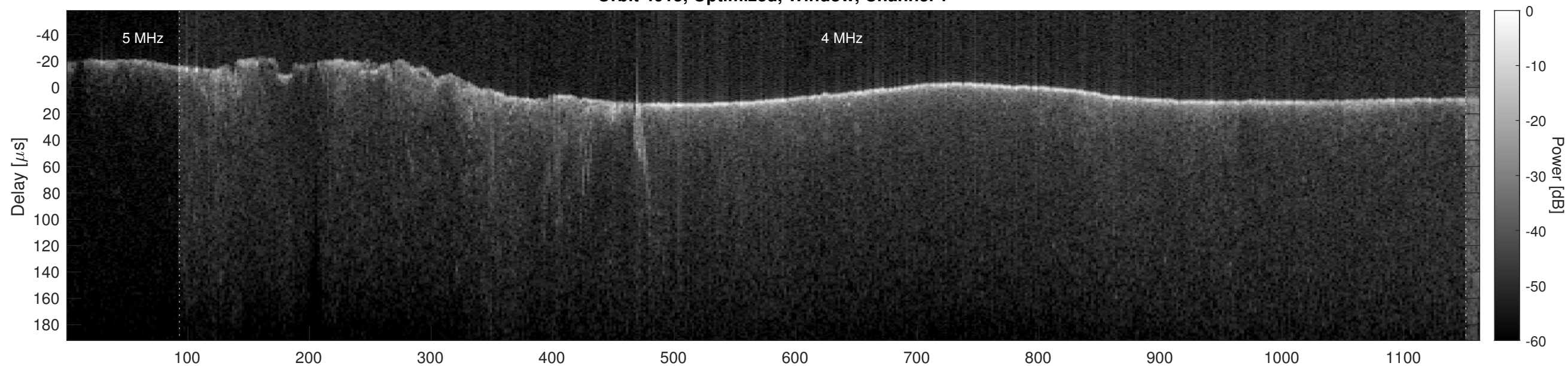
Orbit 4015, Optimized, Window, Channel 2
